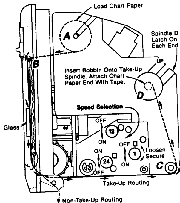
Fig. 9 Take-Up Recorder
