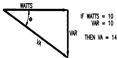
POWER TRIANGLE
